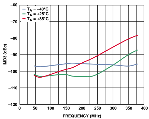
Figure 17. Two-Tone Output IMD3 vs. Frequency, Three Temperatures
