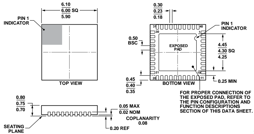
COMPLIANT TO JEDEC STANDARDS MO-220-WJJD. Figure 66. 40-Lead Lead Frame Chip Scale Package [LFCSP_WQ] 6 mm × 6 mm Body, Very Very Thin Quad (CP-40-10) Dimensions shown in millimeters
